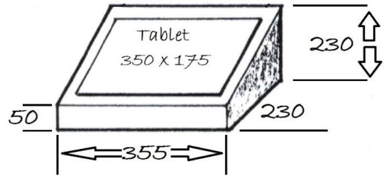
CHILDS TILTED PLAQUE CP - ROWS A~P
